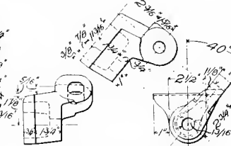
Figs. 4690-2. BRACKET FOR DEAD-LEVER GUIDE (1).
